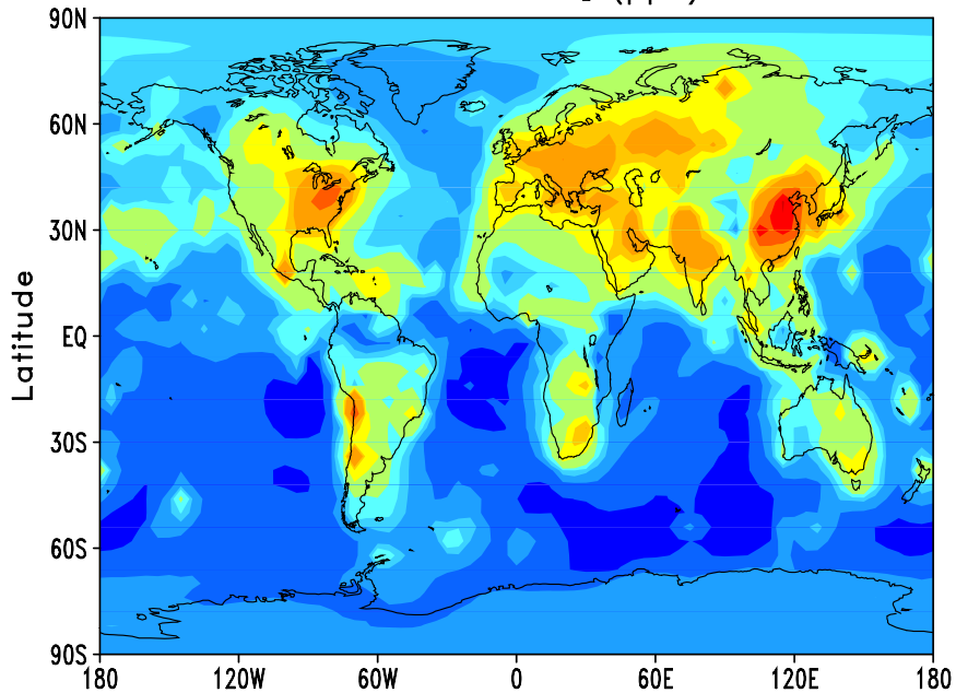
2005 L1-7 SO 2 (ppb)
