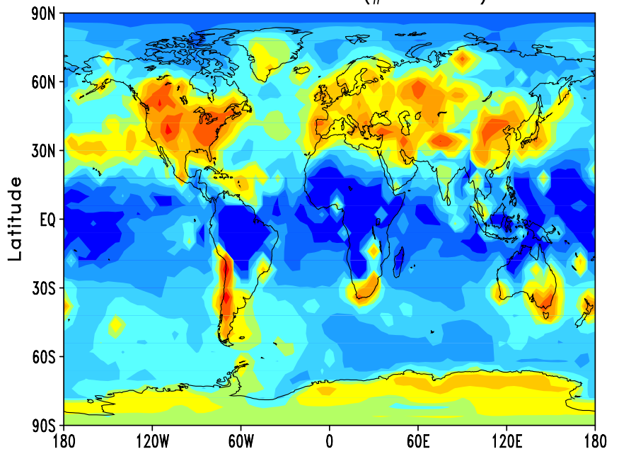
2005 L1-7 JIMN (# cm -3 s -1 )
